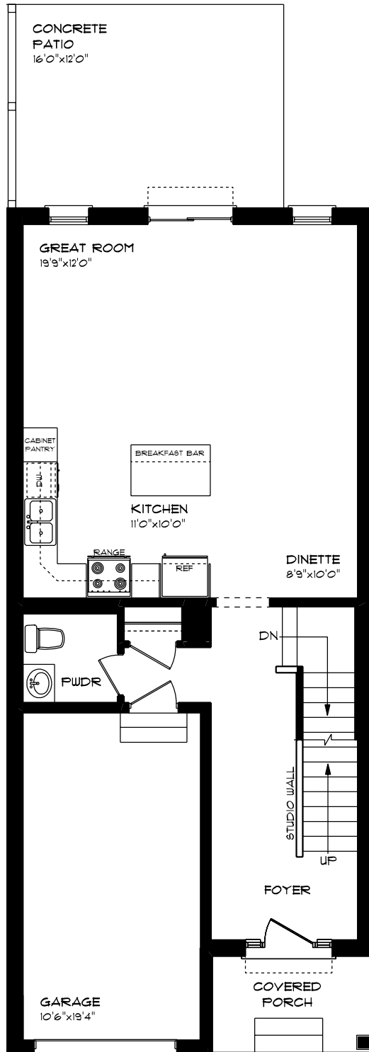
SHELTON - 4 BEDROOM MUN. #23 - 249 RENAISSANCE DRIVE MAIN FLOOR PLAN APPROX. 118 SQ. FT.
