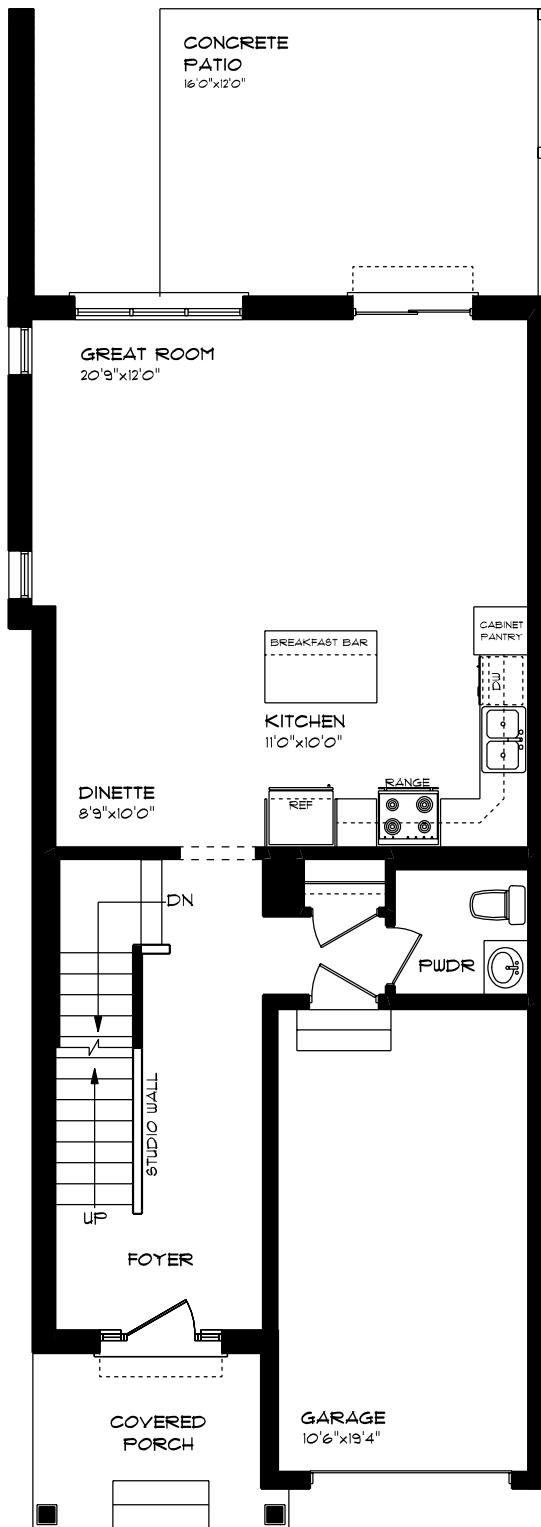
SHELTON - 4 BEDROOM MUN. #85 - 249 RENAISSANCE DRIVE MAIN FLOOR PLAN APPROX. 792 SQ. FT.
